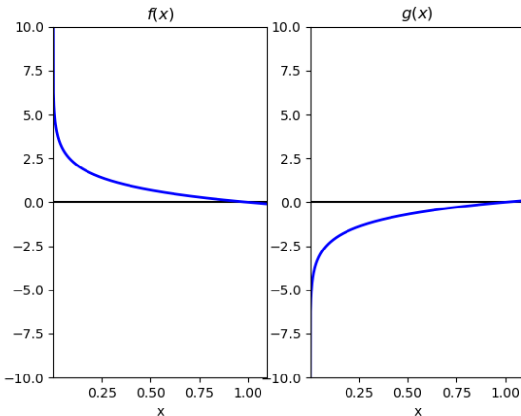
Figure 1: Different possible cost functions
