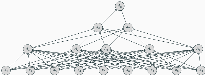
Figure 1: Three-layer neural network for predicting sunshine from three features per day. For a period of time, like Monday, Tuesday, Wednesday, x_1, x_2, x_3 would be features for Monday (e.g., humidity, max temperature, min temperature), x_4, x_5, x_6 for Tuesday, and x_7, x_8, x_9 for Wednesday.
