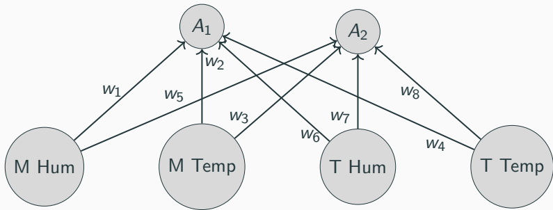
Figure 2: Feed-forward neural network basic prototype
