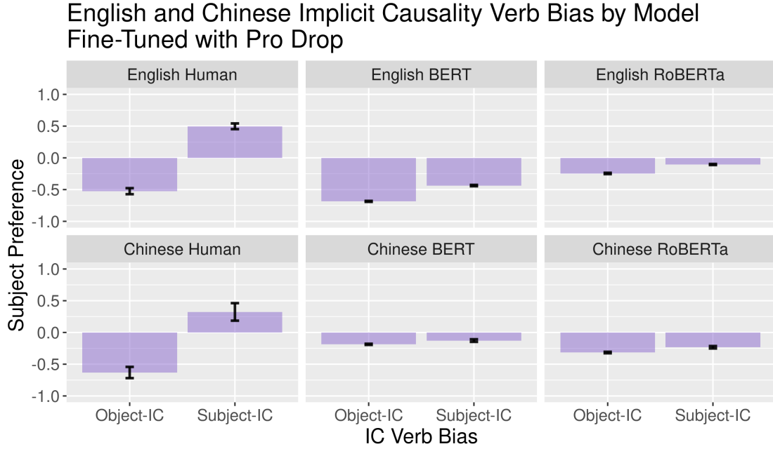
Figure 3.7: Subject preference after fine-tuning on sentences with pro drop (i.e. no subject pronoun). Results are grouped by implicit causality verb type for humans (English is from Ferstl et al., 2011; Chinese is from Hartshorne et al., 2013), English BERT and RoBERTa, and Chinese BERT and RoBERTa. A value of 1.0 corresponds to a complete preference for pronouns agreeing in gender with the subject (i.e. a subject bias), and a value of -1.0 corresponds to a complete preference for pronouns agreeing with the object (i.e. an object bias). Error bars are 95% confidence intervals.
